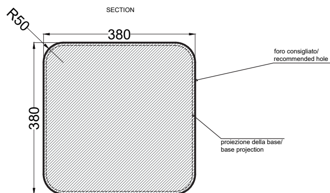
SECTION
