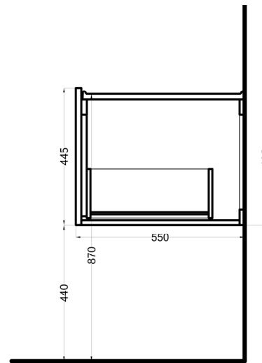
SIDE SECTION
