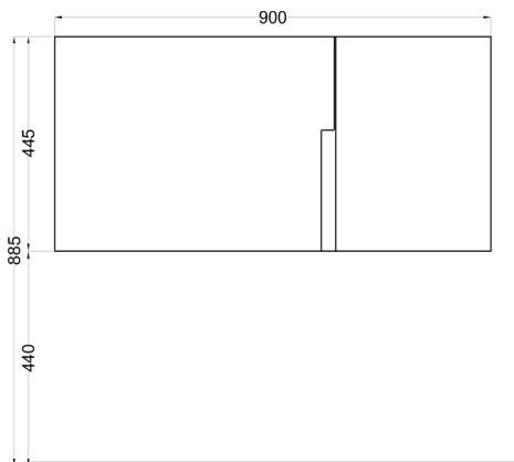
FRONT 1
