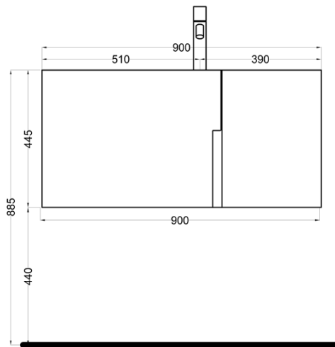
FRONT 2
