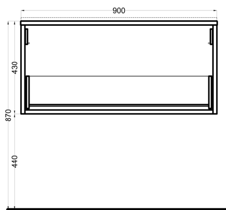
FRONT SECTION
