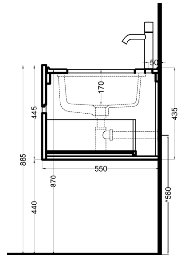
SIDE SECTION
