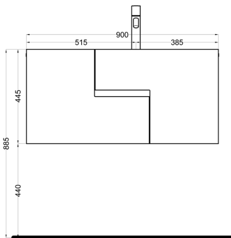
FRONT 1
