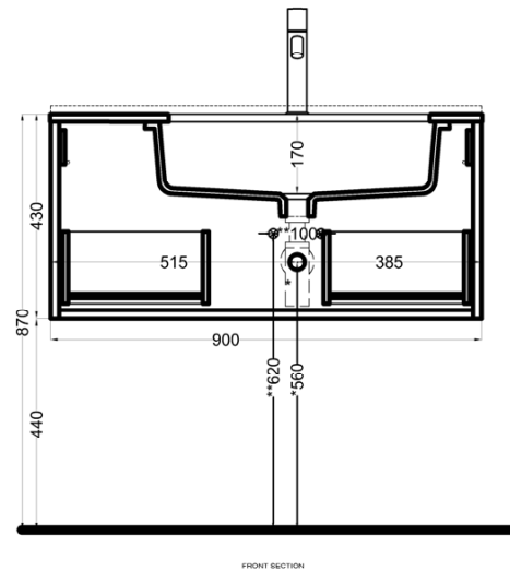
FRONT SECTION
