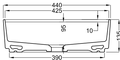
A - A SECTION
