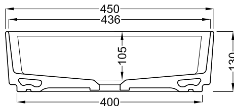
A - A SECTION
