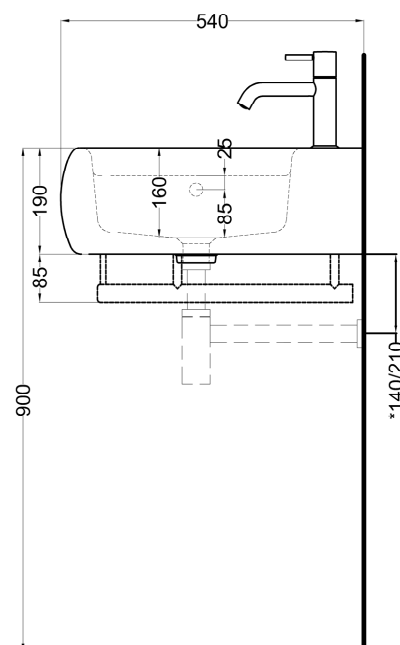
LATERAL VIEW
