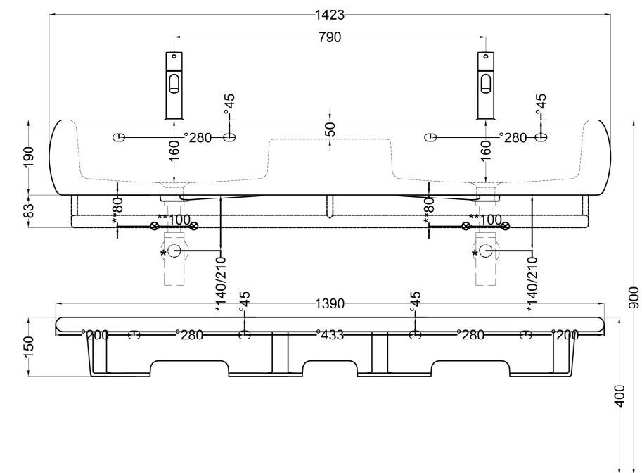
FRONT
